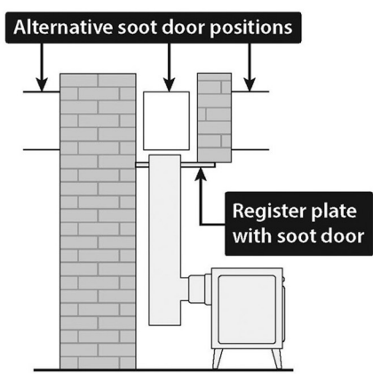
Horizontal register plate with rear flue connection
