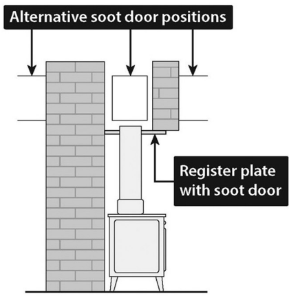
Horizontal register plate with top flue connection
